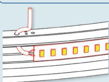
1. Install FlexLED strip inside the profile.
