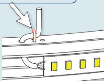
2. Solder wire to the FlexLED strip.
