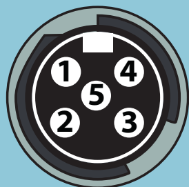
5-Pin Female DC Connector
